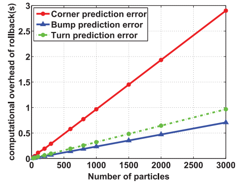
Fig. 15. Latency by different rollback types and numbers of particles.
