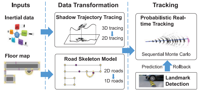
Fig. 1. In the data transformation stage, the shadow trajectory tracing simplifies 3D vehicle tracing into 2D shadow tracing while road skeleton model further reduces 2D tracing into 1D. In the tracking stage, VeTrack represents vehicle states probabilistically and uses a Sequential Monte Carlo framework for robust tracking. It also uses landmark detection to calibrate vehicle states and prediction/rollback for minimum latency.
