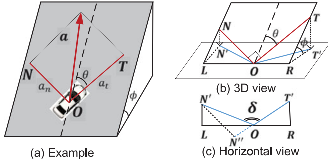
Fig. 5. (a) Driving a vehicle O on the slope with acceleration a . (b) 3D view, the inclination angle of slope is \phi , and vehicle's heading direction \overline{OT} is at angle \theta to the direction of slope. (c) Horizontal plane view.
