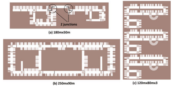
Fig. 10. Floor maps of three underground parking lots: (a) university campus: 180 m \times 50 m with 79 parking spots, 12 bumps, and 11 turns. (b) Office building: 250 m \times 90 m with 298 parking spots, 19 bumps, and 10 turns. (c) Shopping mall: Three-level 120 m \times 80 m with 423 parking spots, 10 bumps, and 27 turns. The chosen parking spots and entrance are marked for each lot.
