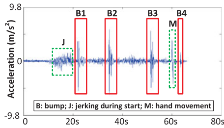
Fig. 8. Acceleration along the Z -axis. There are starting acceleration ( J ), four bumps ( B1 - B4 ), and one hand movement ( M ) along the trajectory.
