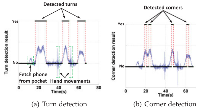
Fig. 9. Turn and corner detection. (a) Three turn periods are correctly detected, even there are several different hand movements. (b) Four corners are correctly separated, even when only three turns are detected.
