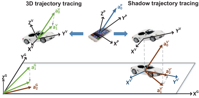
Fig. 4. Illustration of 3D trajectory tracing and shadow trajectory tracing. Left part: 3D trajectory tracing, a_0^P \rightarrow a_0^V \rightarrow a_1^V \rightarrow a_1^G ; right part: Shadow trajectory tracing, a_0^P \rightarrow a_0^V \rightarrow a_1^V \rightarrow a_2^V \rightarrow a_2^G .
