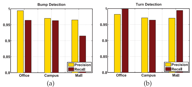
Fig. 13. Precision and recall of bump and turn detection in three different garages.
