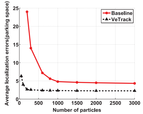
Fig. 16. Tracking error by numbers of particles.
