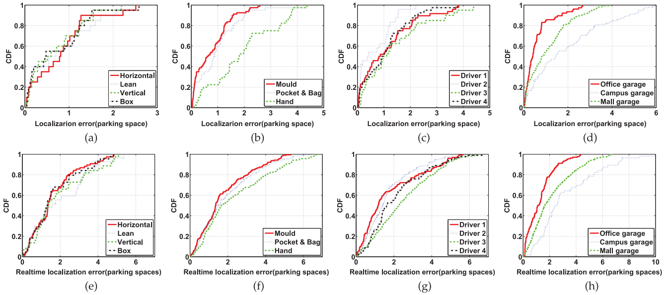
Fig. 17. Final parking location errors (1st row) and realtime tracking location errors (2nd row). (a) and (e) Four phones in the mould. (b) and (f) In mould, pocket&bag, and hands. (c) and (g) Different drivers. (d) and (h) Different garages.
