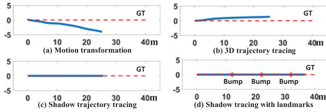
Fig. 2. Illustration of vehicle tracing using different methods: (a) motion transformation, (b) 3D trajectory tracing with gyroscope, (c) shadow trajectory tracing, and (d) shadow trajectory tracing with landmarks.
